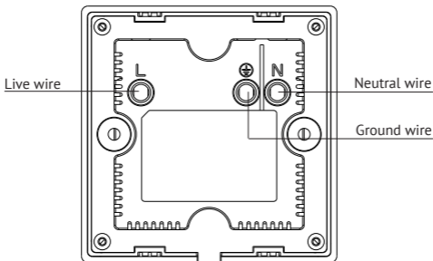
Wiring Diagram
